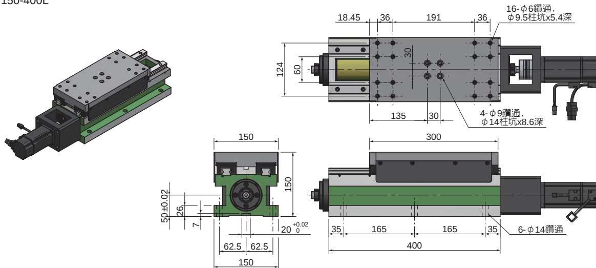
RH150-400L
