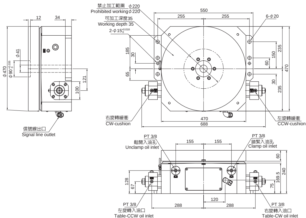
HCT-470
