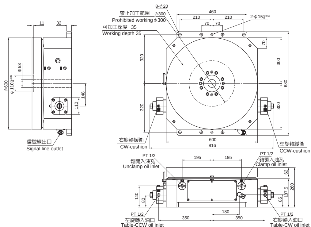
HCT-600
